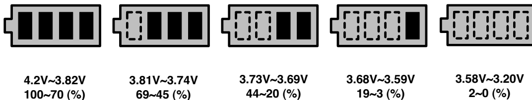
Figure 1.13 U250/KU250 Battery Bar Display(Stand By Condition)
