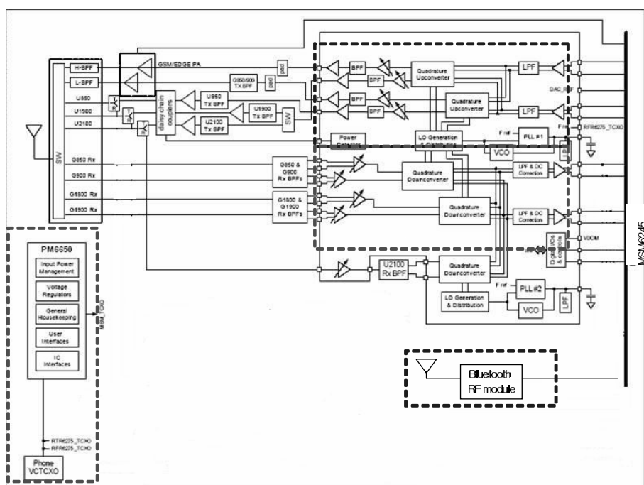
[Fig 1.1] Block diagram of RF part
