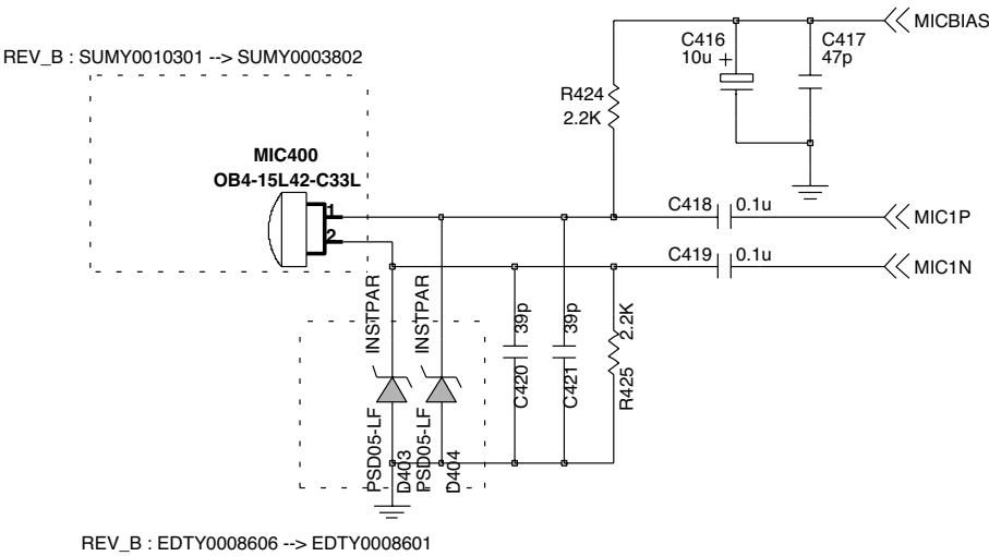
Figure 1.27 Audio part schematics
