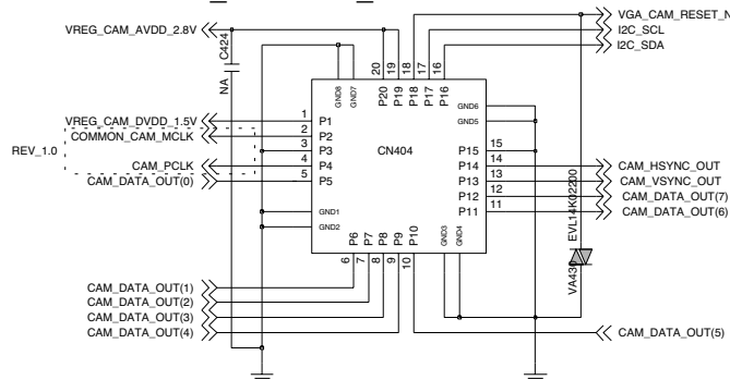
Figure 1.21 Camera Socket Type Connector
